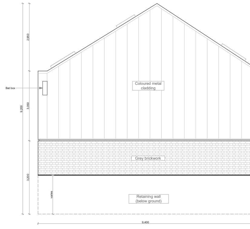
North Elevation
