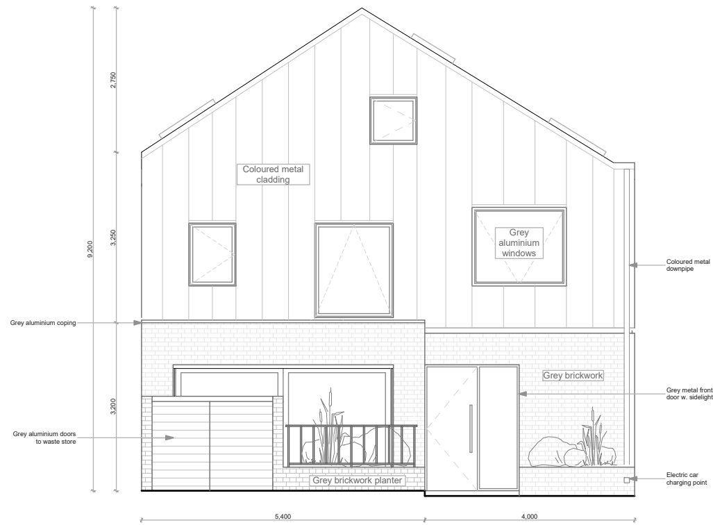
South Elevation
