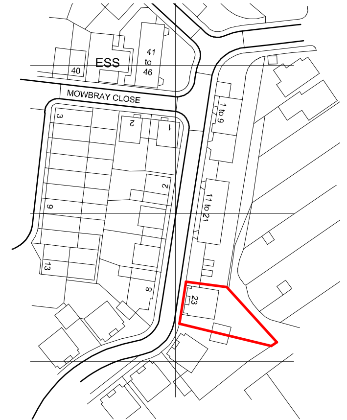
Location Plan 1:1250
