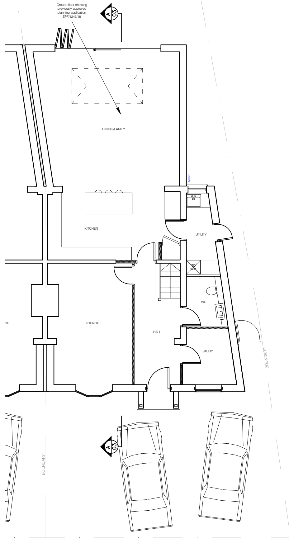
GROUND FLOOR GROUND FLOOR
