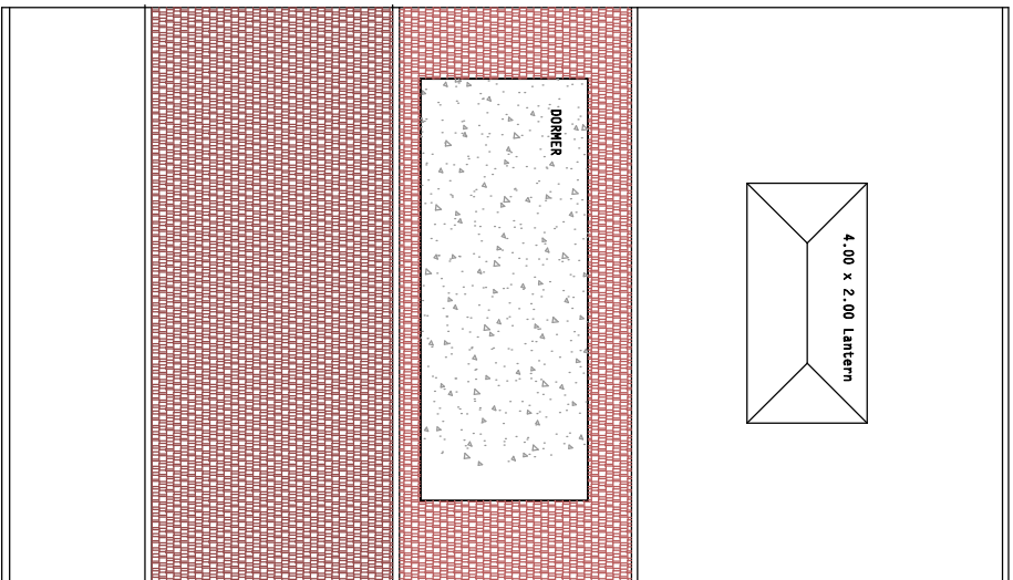
Existing Roof
