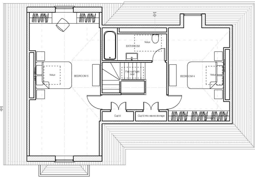
FIRST FLOOR 69sqm/742.7sqft
