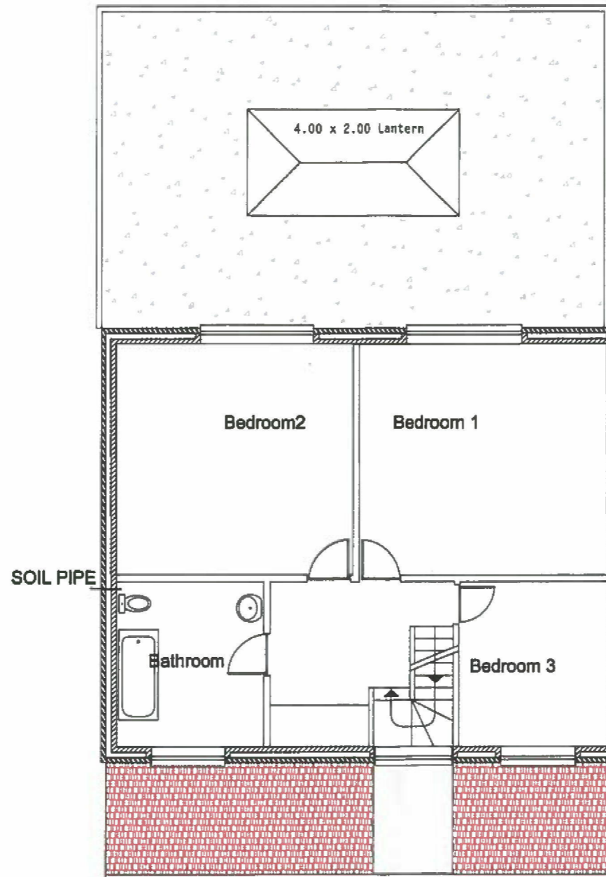
Proposed First
