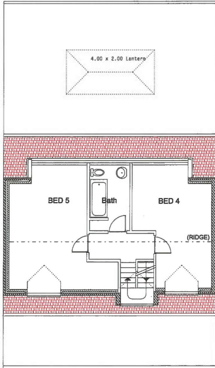
Proposed Loft
