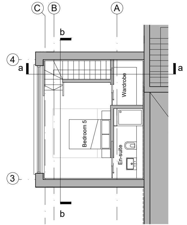
keyplan @ 1:100
