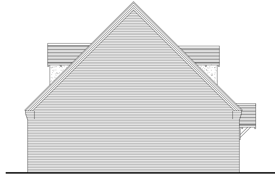
Left Elevation
