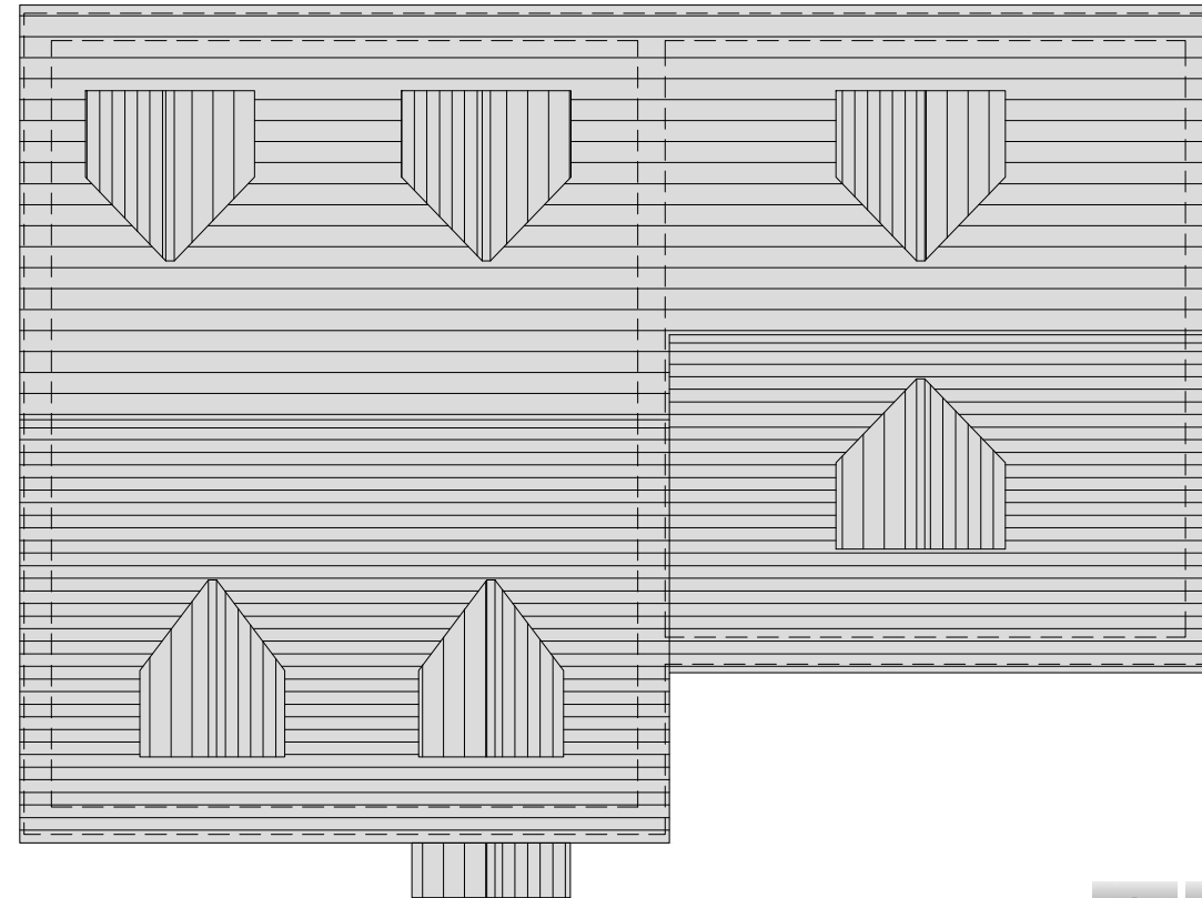
Roof Plan
