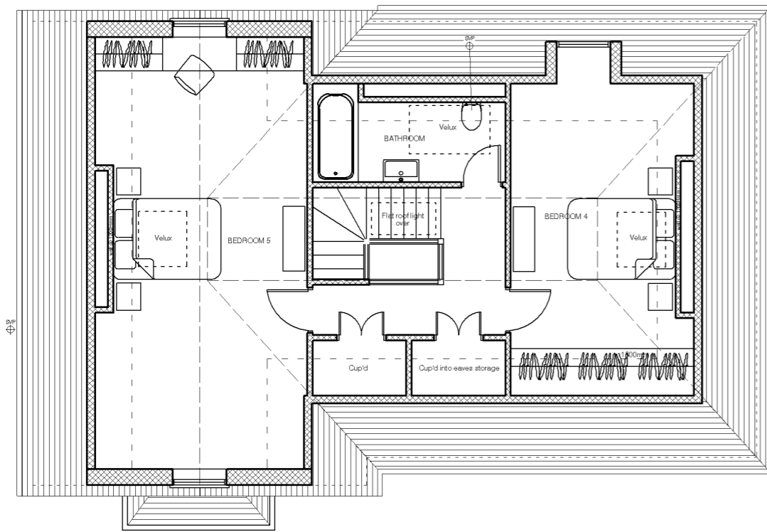
FIRST FLOOR 73.6sqm/792.2sqft
