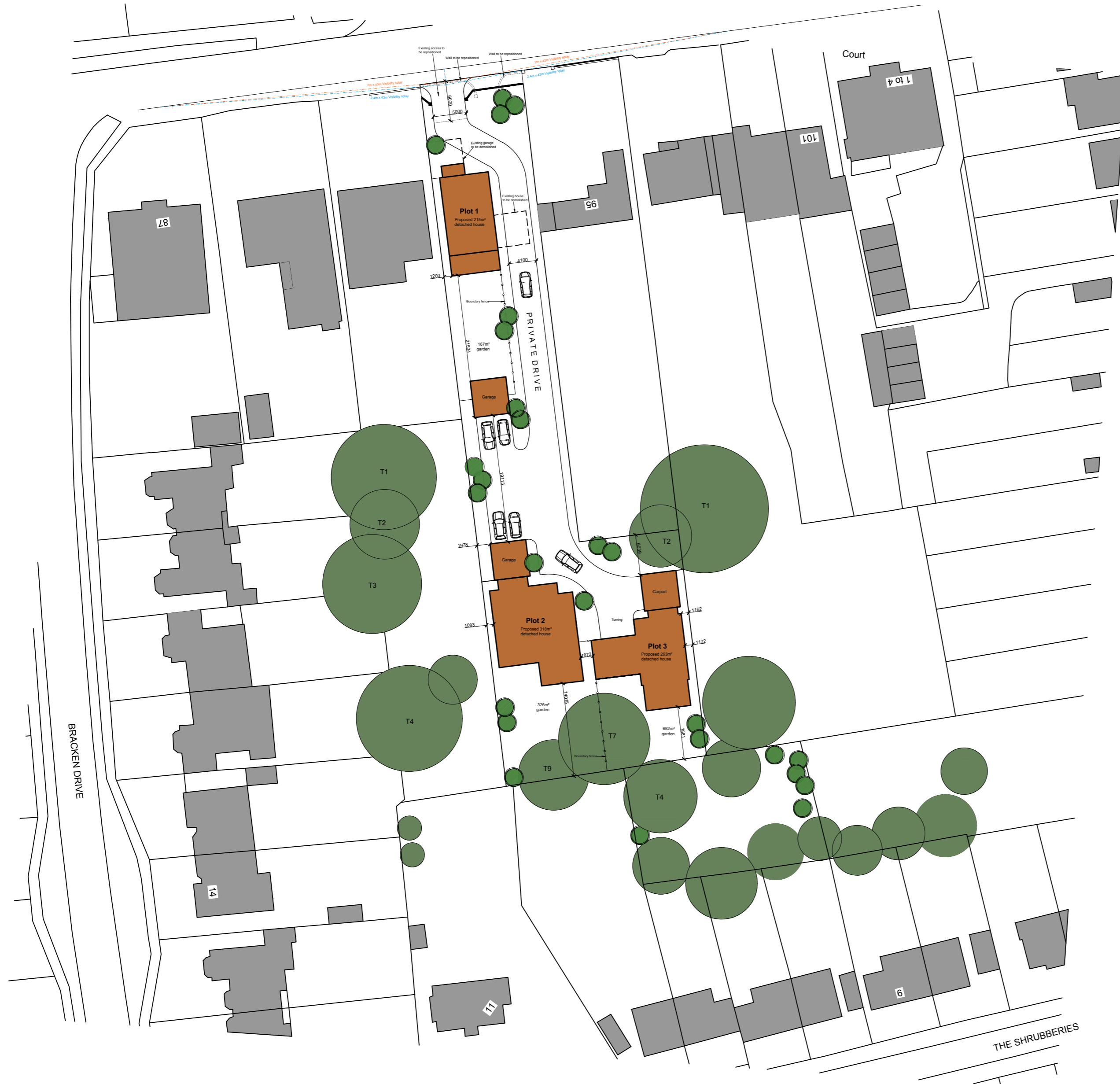
1:200 Site Layout Plan
